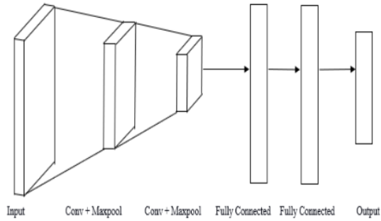
Figure 2 CNN Architecture
